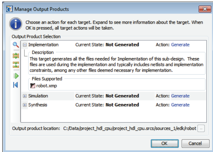
Figure 3-37: Generate Embedded Source Output Products
