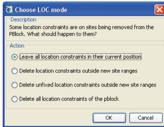
Figure 10-16: Set Pblock Size with LOCs
