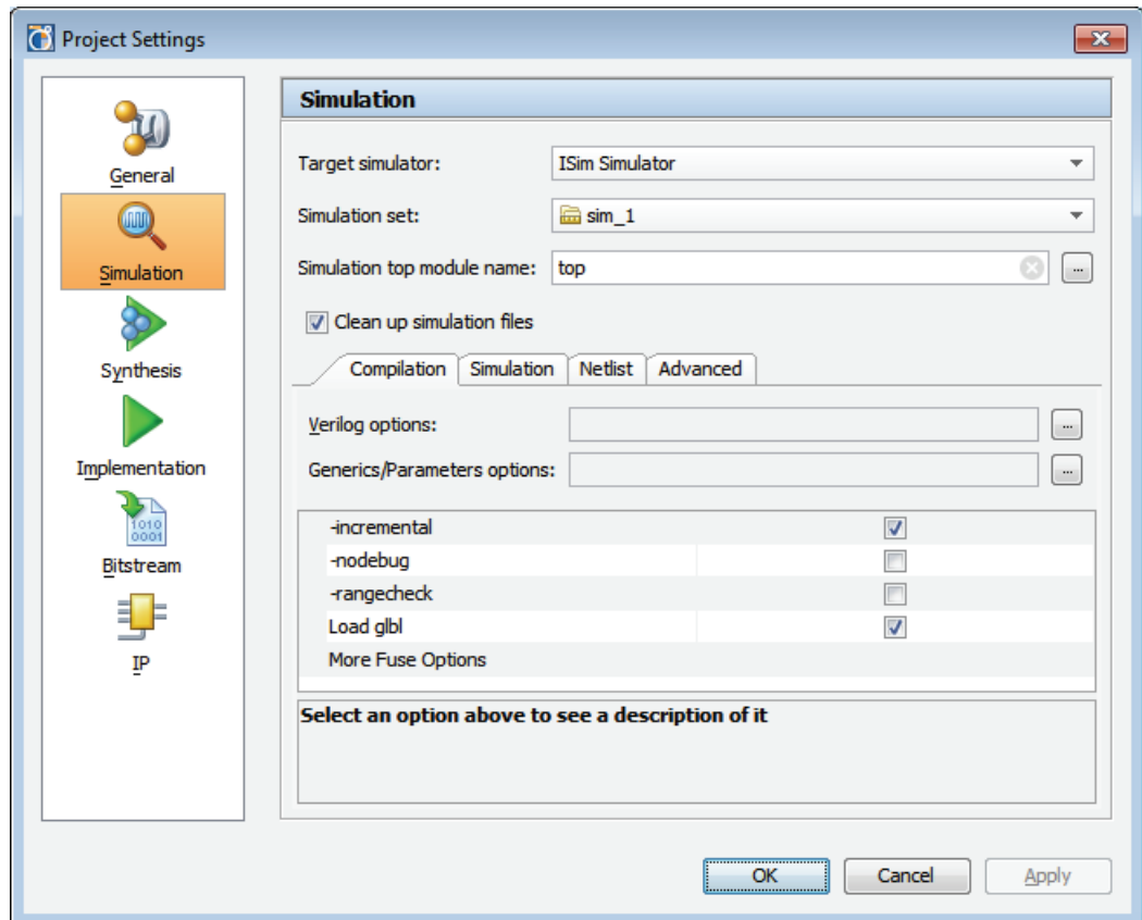
Figure 3-47: Simulation Project Settings
