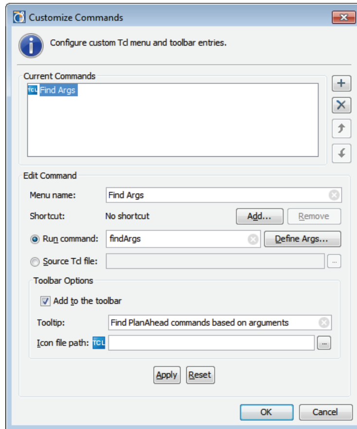
Figure 4-72: Customizing Menu Commands
