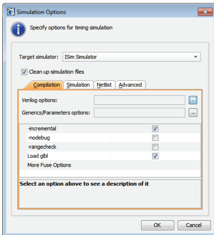
Figure 11-21: Timing Simulation - Compilation Options
