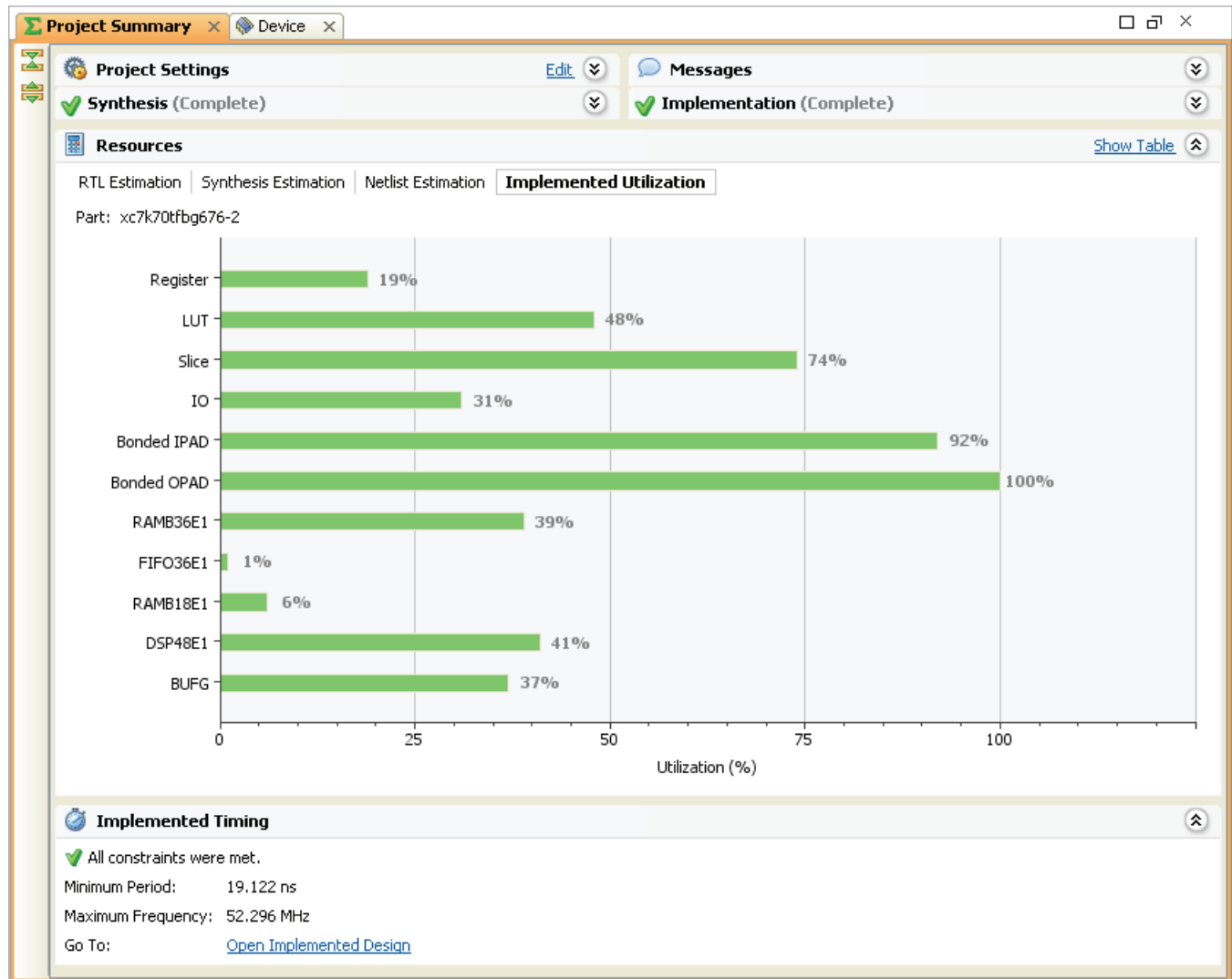
Figure 3-41: Graphical Resource Estimates
