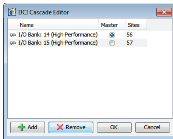
Figure 8-16: Creating a DCI Cascade
