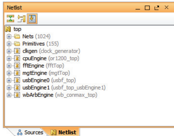
Figure 7-3: Netlist View with Top Module Selected
