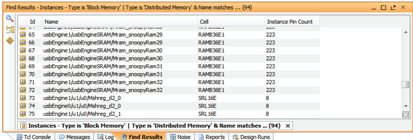
Figure 4-32: Find Results View
