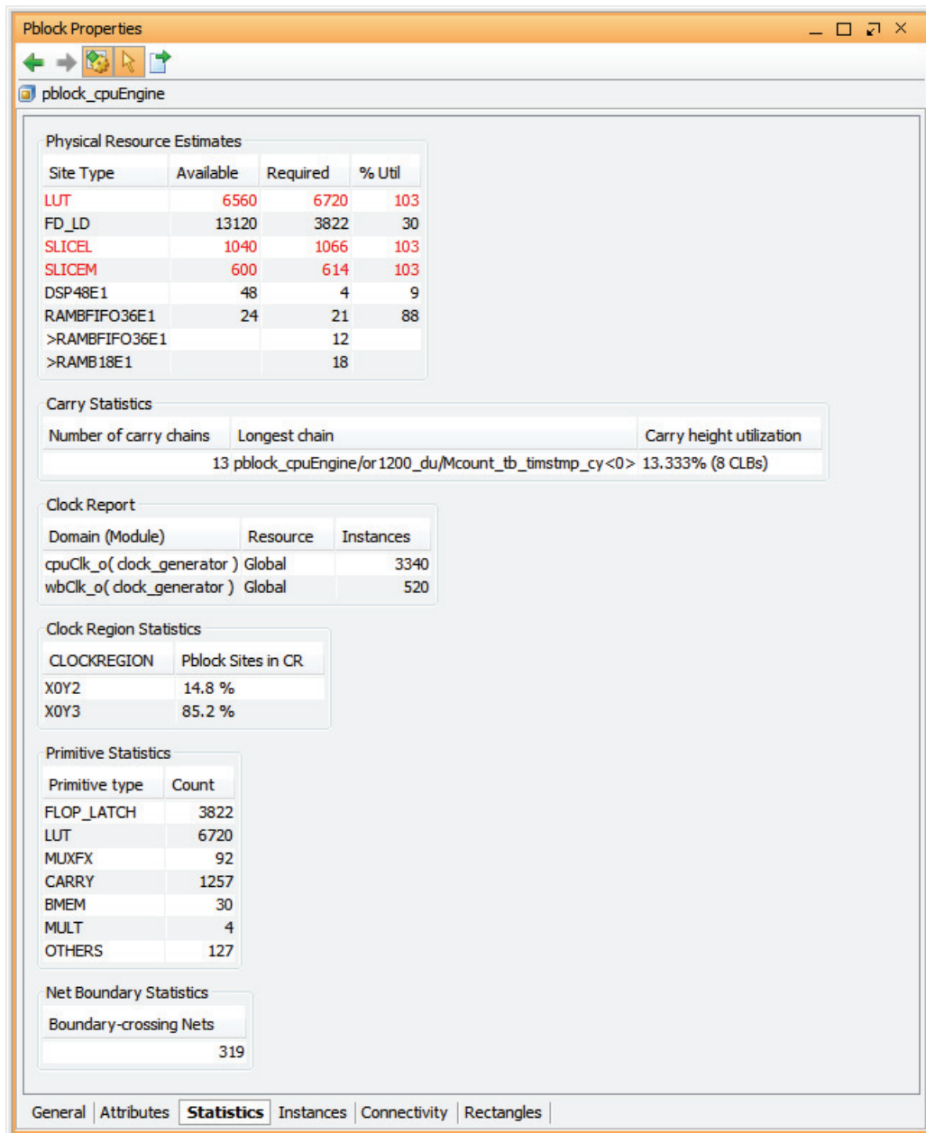
Figure 7-6: Pblock Properties: Statistics Tab
