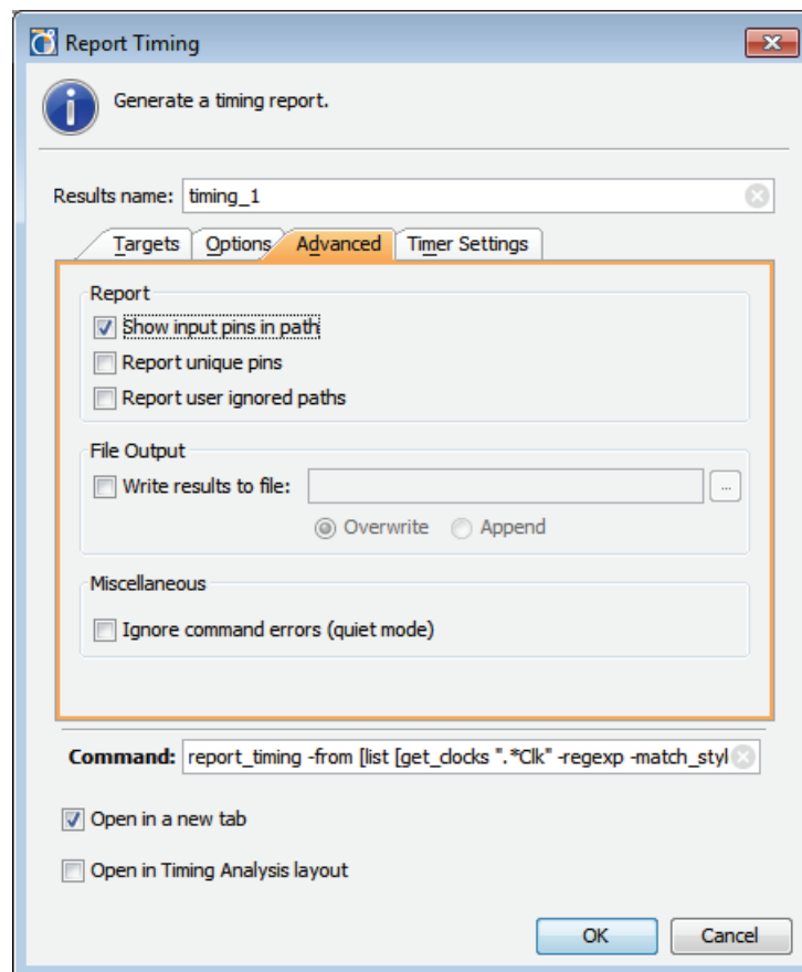
Figure 7-15: Report Timing - Advanced Tab
