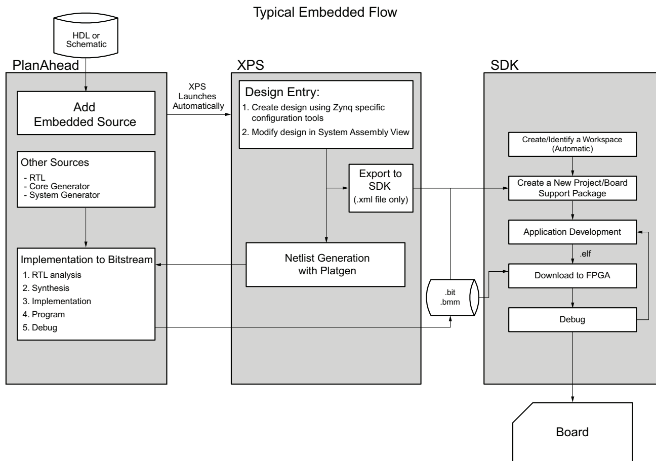
Figure 3-32: Embedded Design Flow
