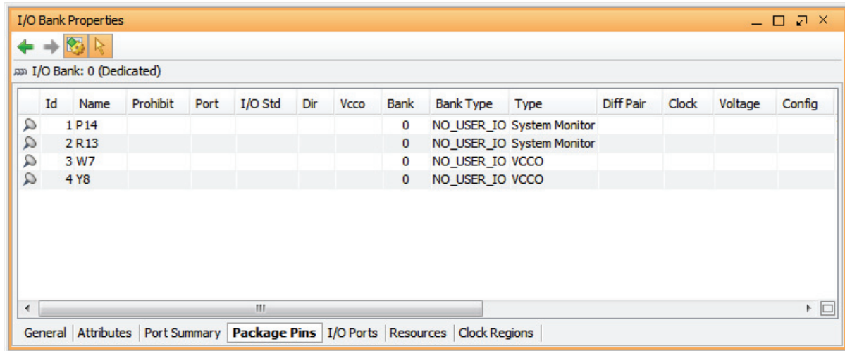
Figure 8-5: Displaying I/O Bank Properties
