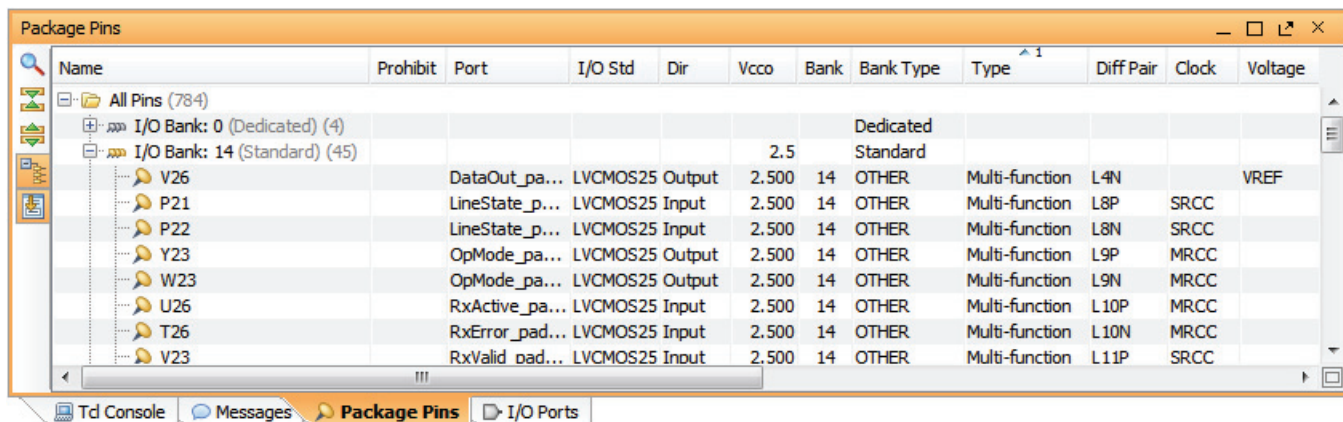
Figure 8-6: Package Pin View
