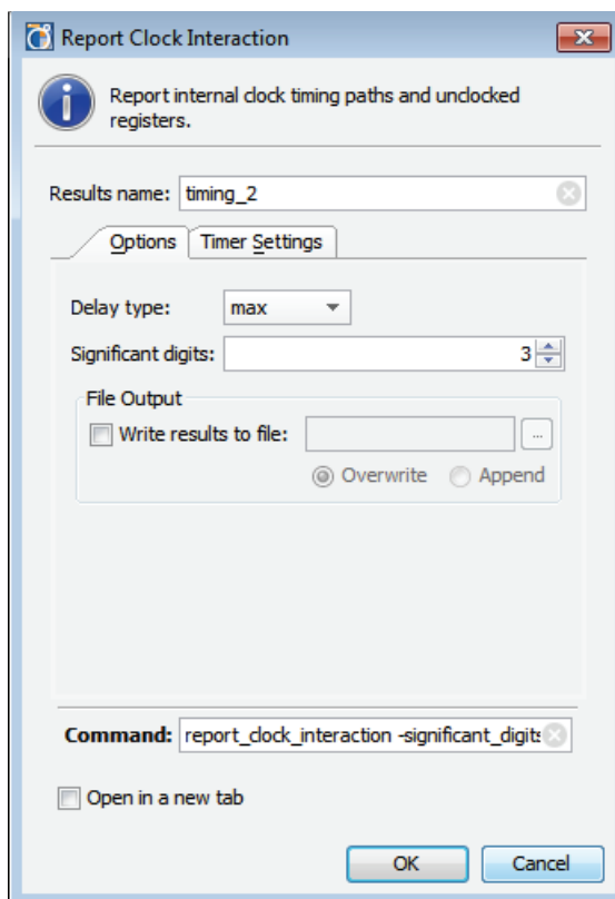
Figure 7-19: Report Clock Interaction - Options Tab
