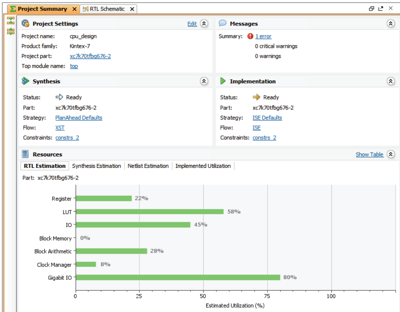
Figure 5-2: Resource Utilization of an Elaborated Design
