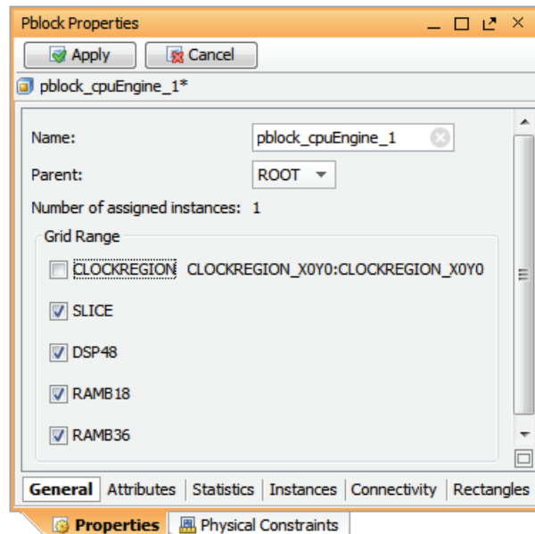
Figure 10-11: Setting AREA_GROUP Range Types
