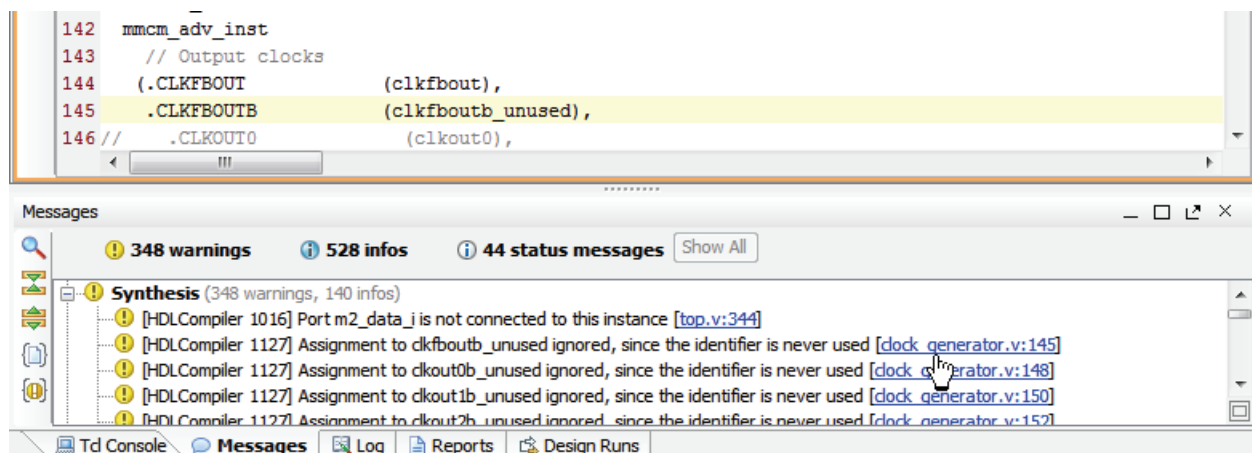
Figure 6-8: Synthesis Message and RTL Source File
