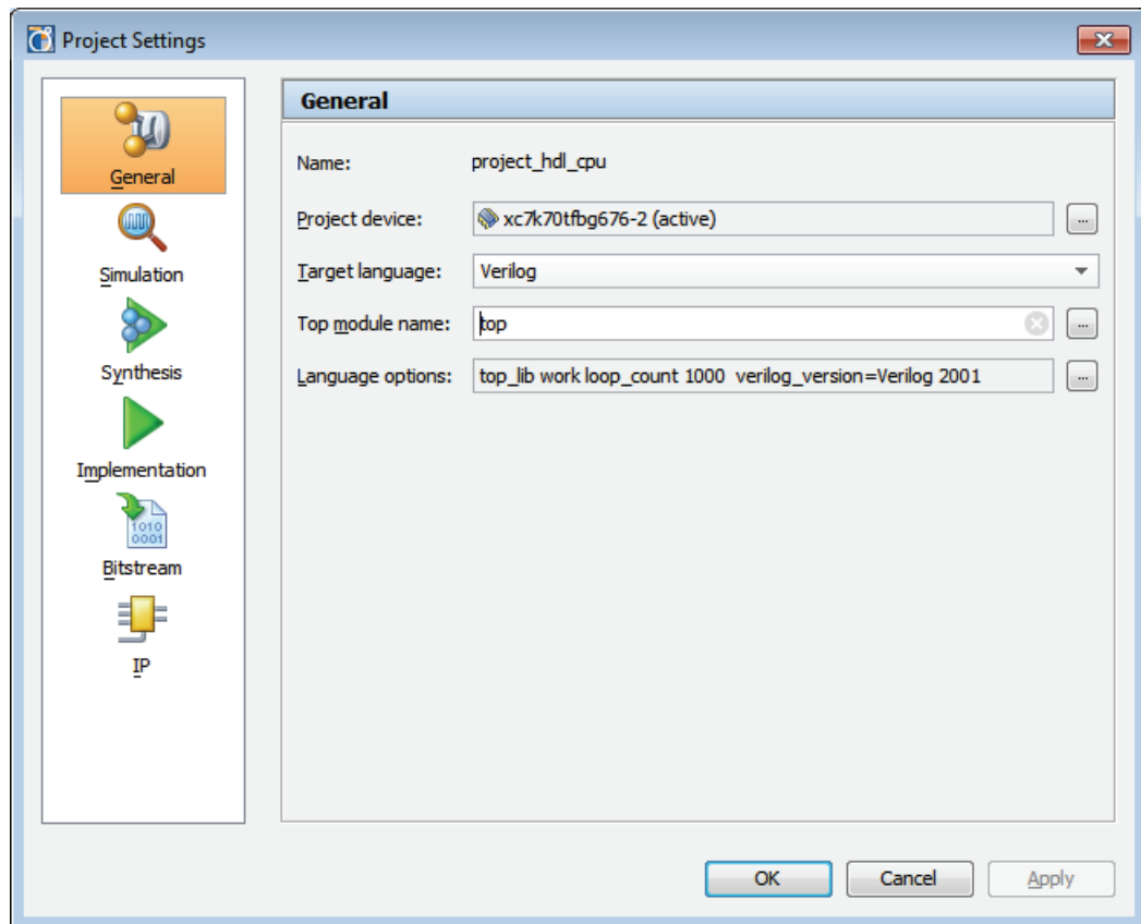
Figure 3-44: General Project Settings
