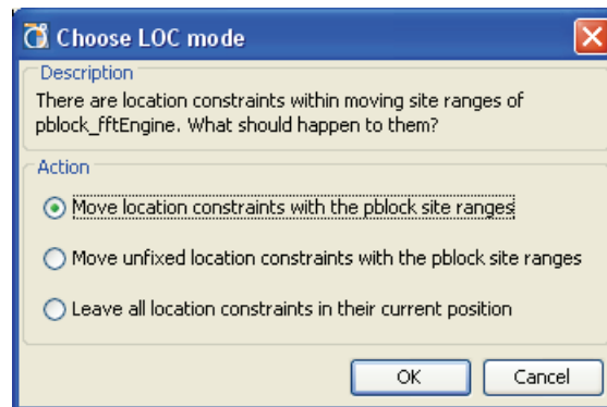
Figure 10-14: Moving Pblocks with LOCs
