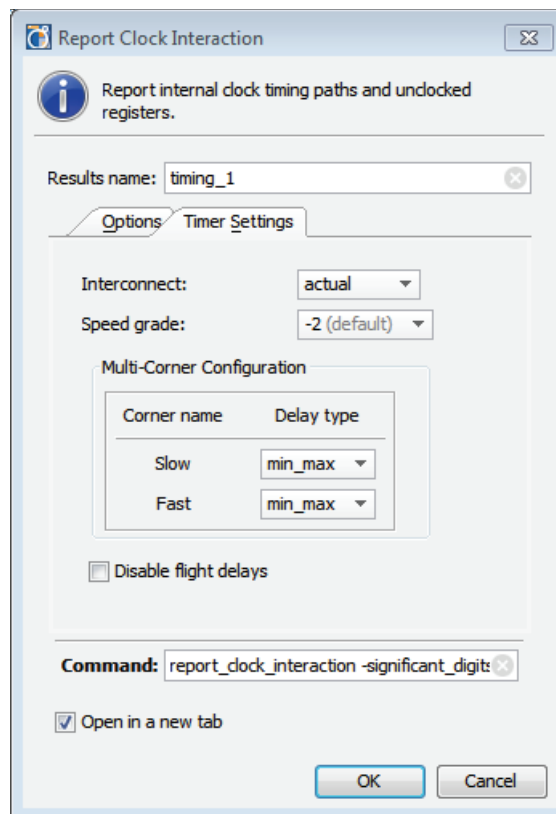
Figure 7-20: Report Clock Interaction - Timer Settings Tab
