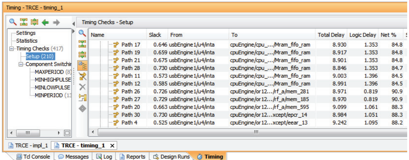
Figure 11-7: Sorted Timing Results and Group by Constraint
