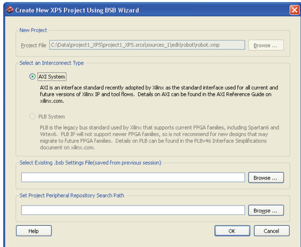
Figure 3-34: Base System Builder
