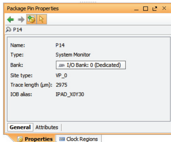
Figure 8-2: Package Pin Properties
