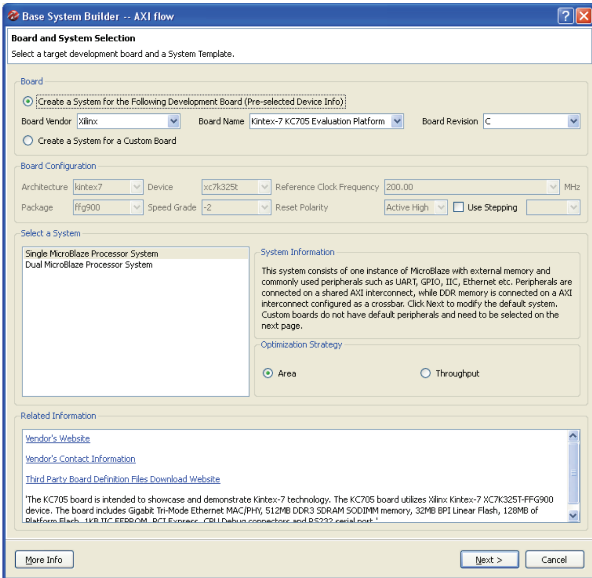
Figure 3-35: Board and System Selection
