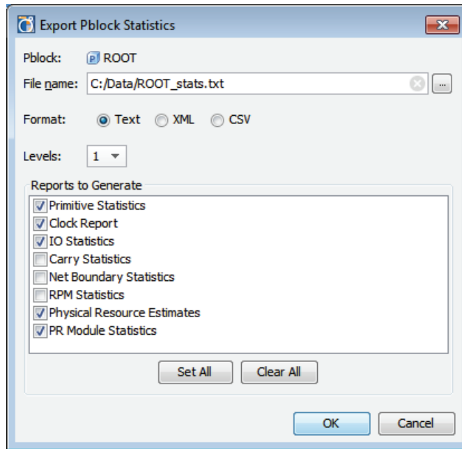
Figure 7-7: Export Netlist Resource Statistics
