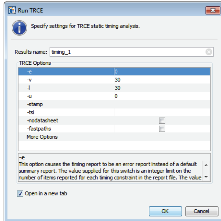
Figure 11-5: Run TRCE Dialog Box
