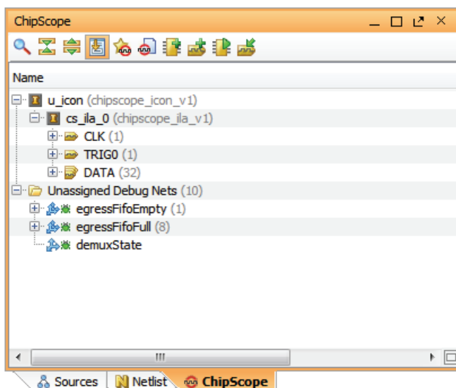
Figure 12-3: Unassigned Nets List in ChipScope Window
