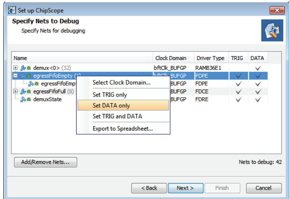
Figure 12-4: Specifying Debug Nets and Clock Domains
