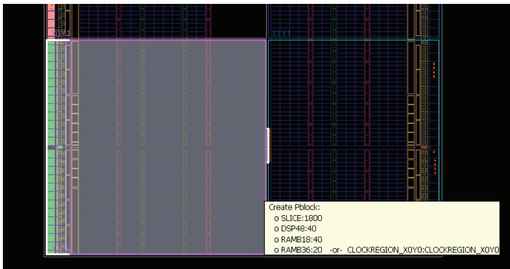
Figure 10-6: Creating Clock Region Pblocks
