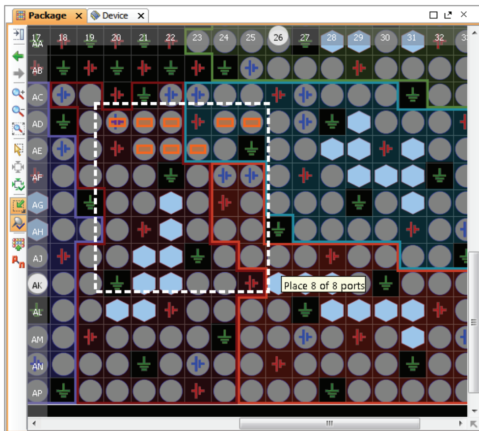
Figure 8-23: Placing I/O Ports in an Area
