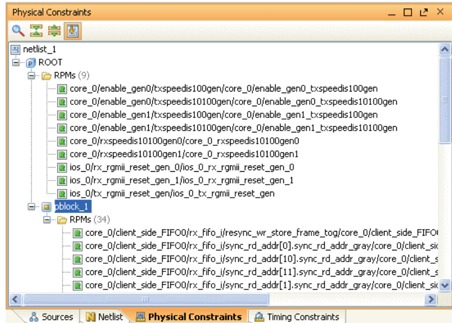
Figure 7-24: Displaying Relatively Placed Macros “RPMs”
