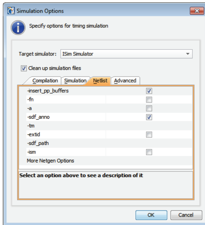
Figure 11-23: Timing Simulation - Netlist Options
