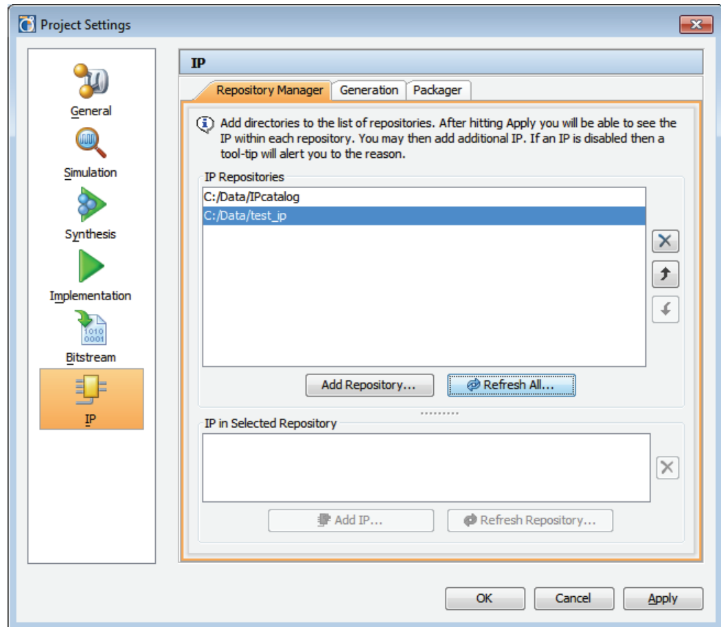
Figure 3-51: IP Catalog Project Settings
