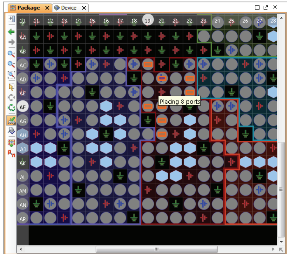
Figure 8-22: Placing I/O Ports in I/O Banks
