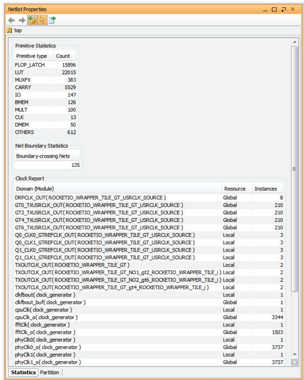
Figure 7-4: Netlist Resource Statistics
