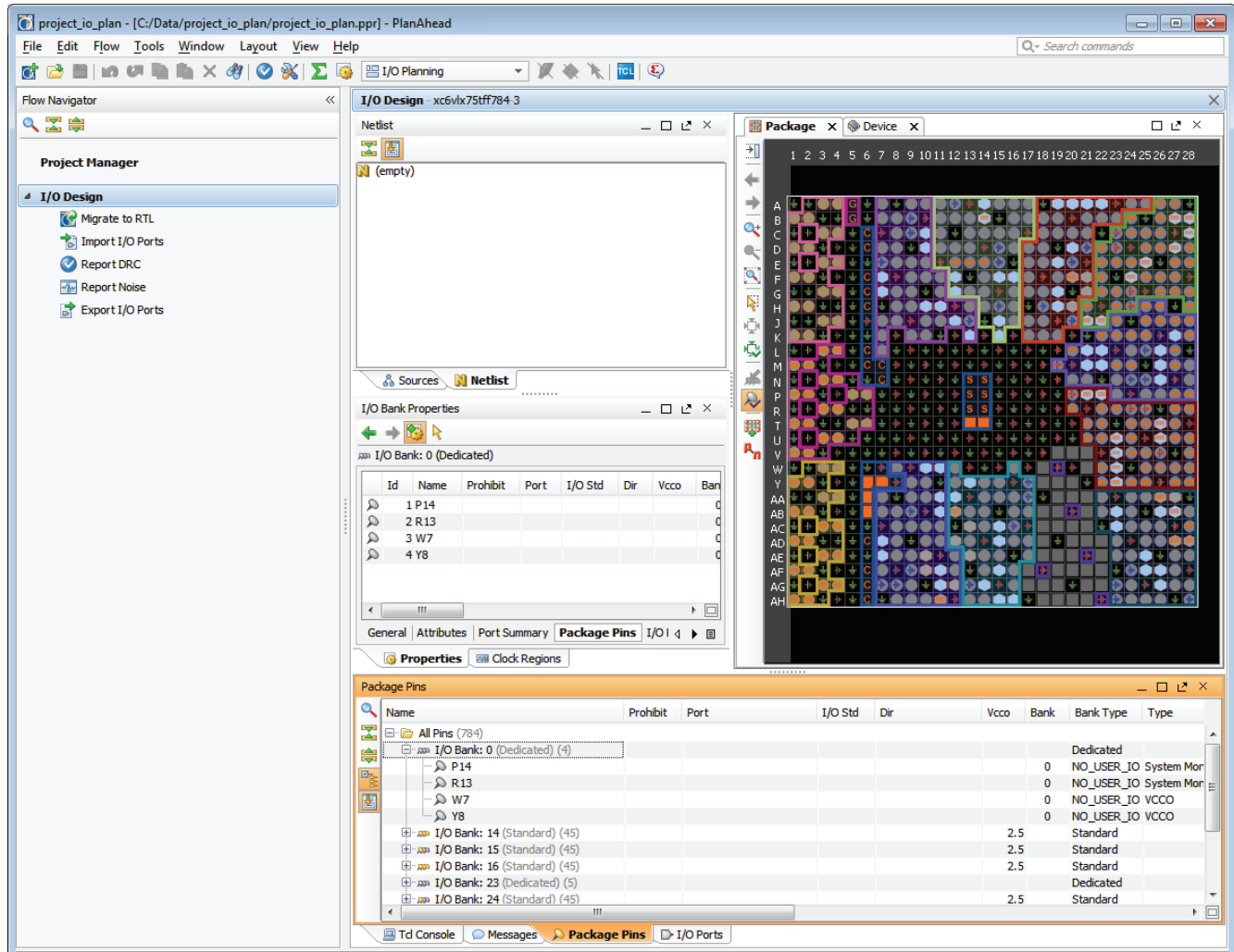
Figure 8-1: I/O Planning Environment
