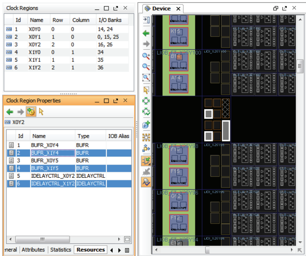
Figure 8-4: Viewing Clock Region Resources
