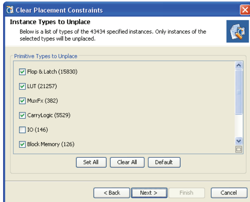
Figure 10-29: Unplace Instance Types
