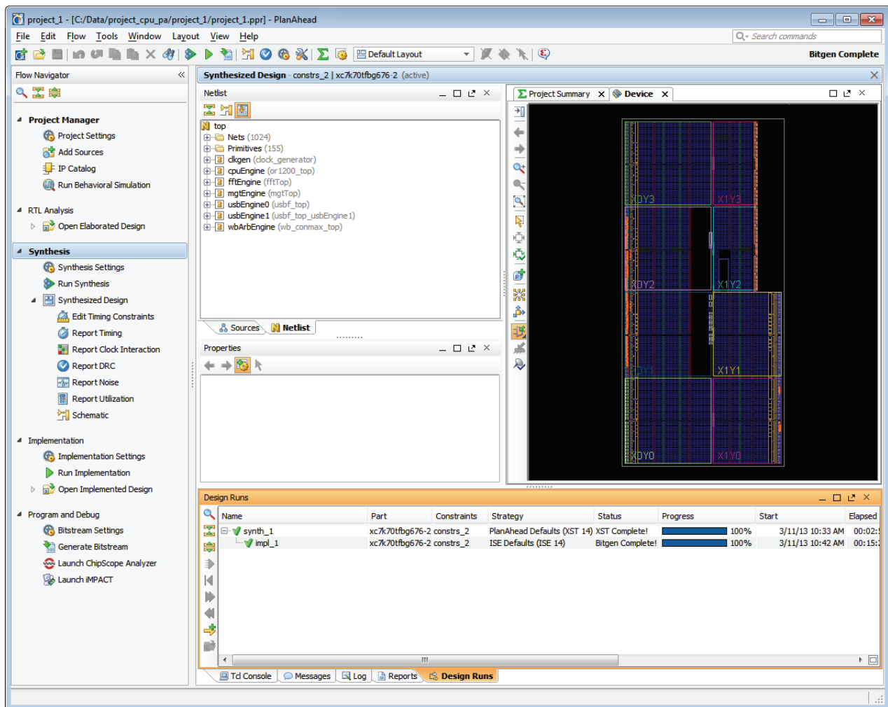
Figure 2-9: Open Synthesized Design
