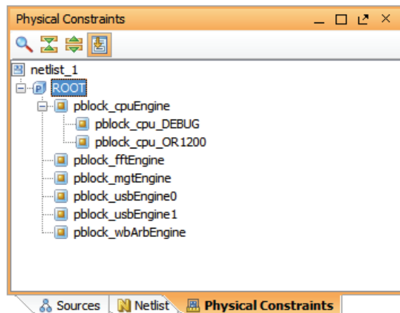
Figure 7-23: Physical Constraints View
