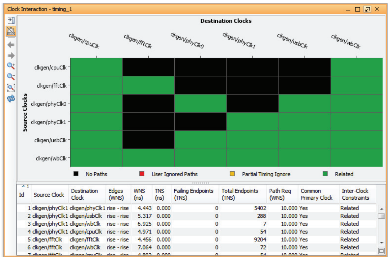
Figure 7-21: Clock Interaction Report
