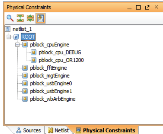
Figure 7-5: Physical Constraints View with ROOT Selected
