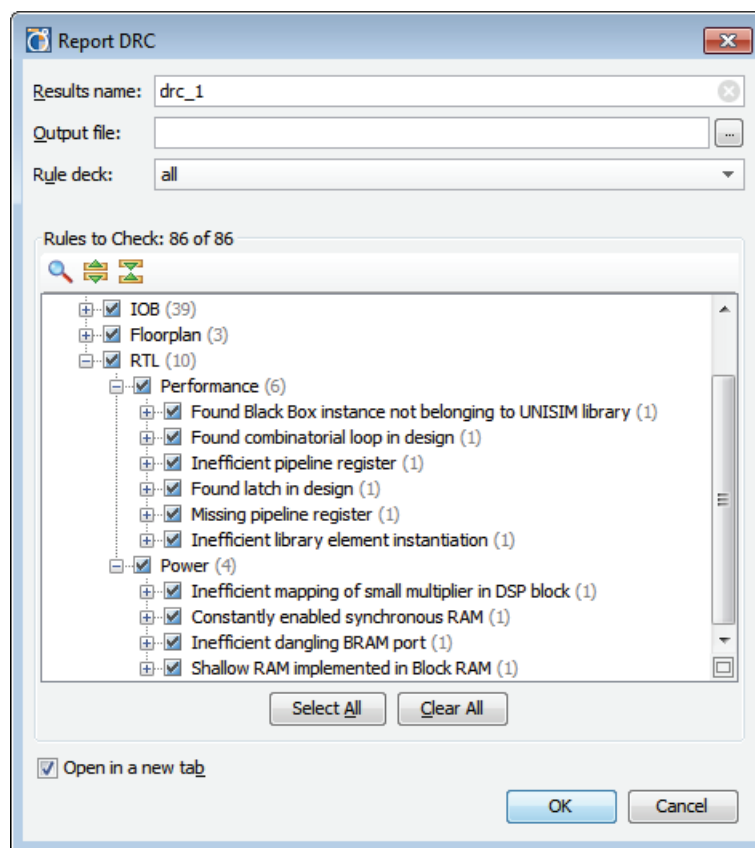
Figure 5-9: Run Design Rule Checker Dialog Box
