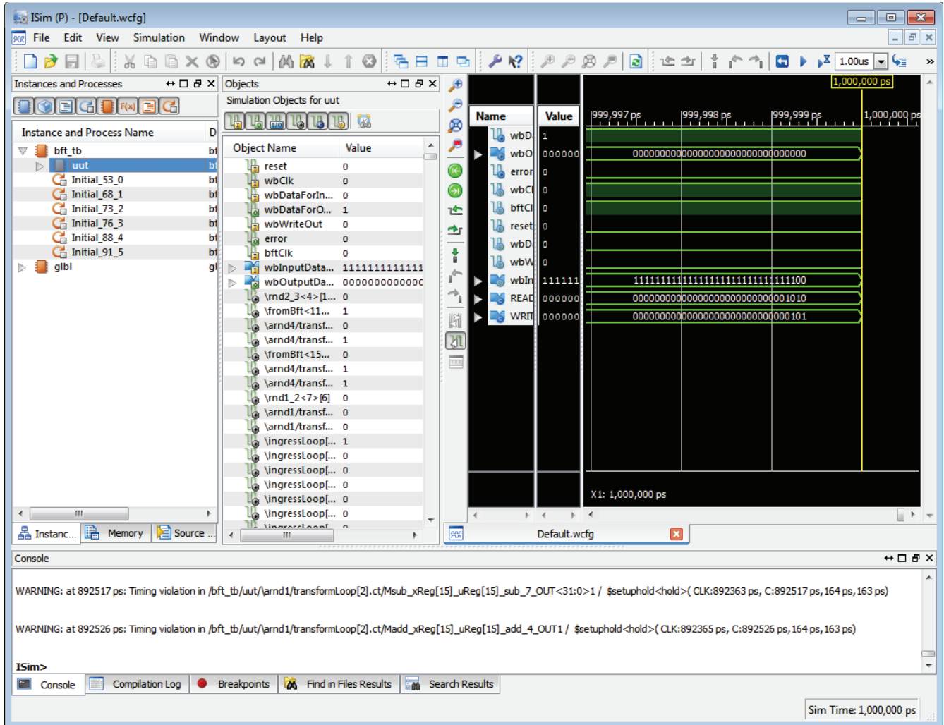
Figure 5-8: ISim User Interface
