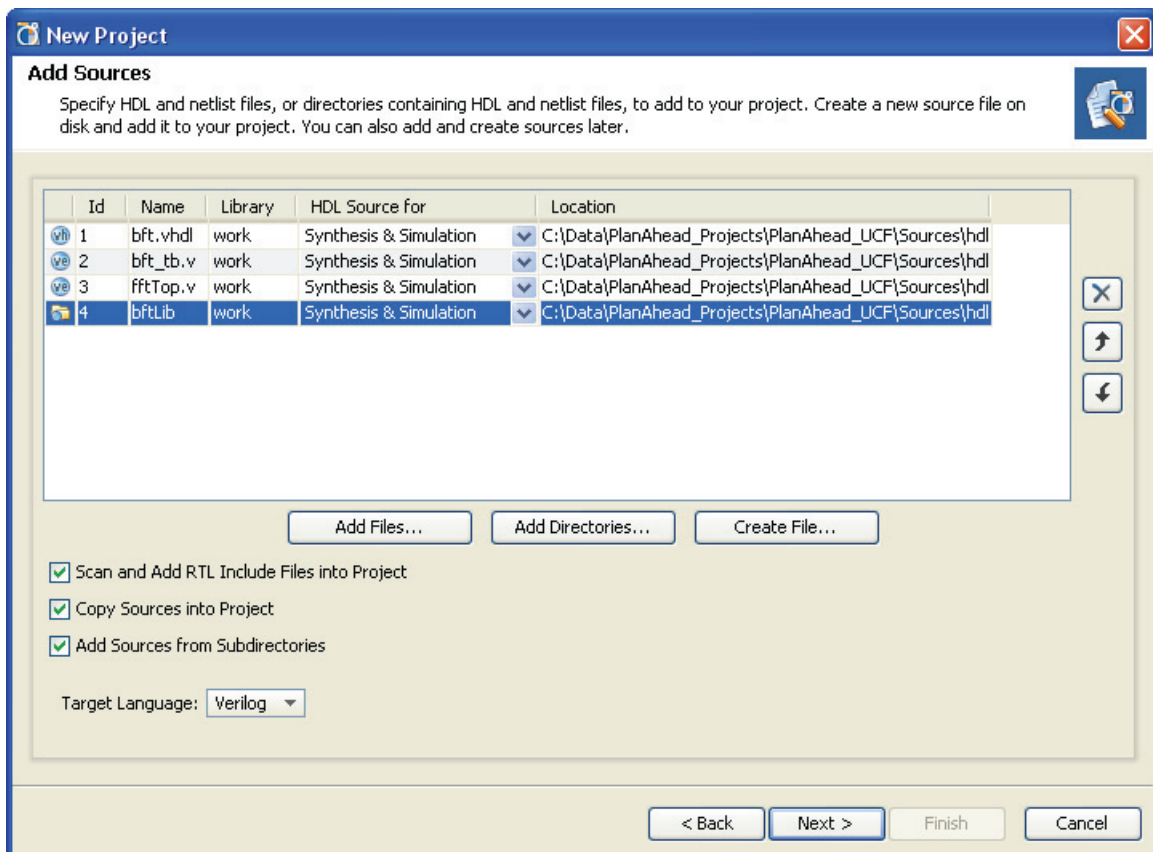
Figure 3-3: New Project Wizard: Add Sources
