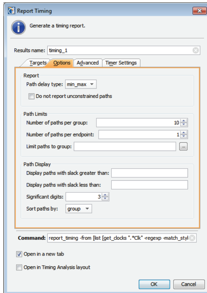
Figure 7-14: Report Timing - Options tab
