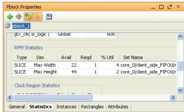
Figure 7-25: RPM Utilization Statistics for Pblocks
