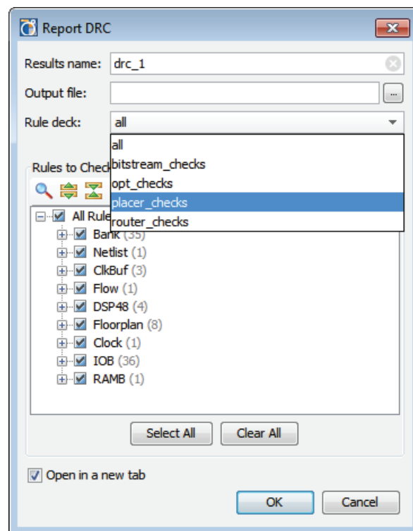
Figure 8-28: Run DRC Dialog Box: I/O Pin and Clock DRC Rules
