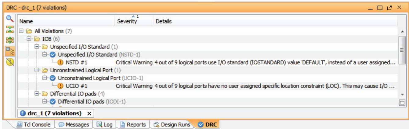
Figure 8-29: Highlighting DRC Violations
