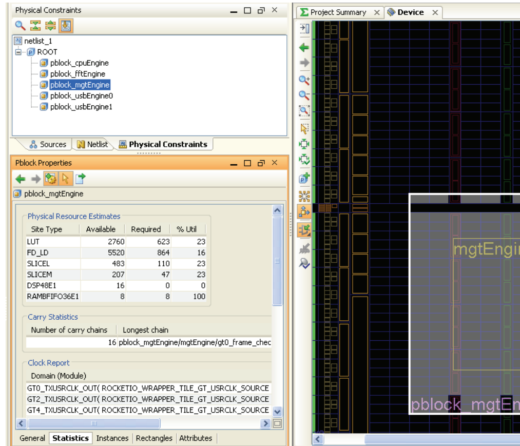
Figure 10-12: Pblock Shading Reflects Logic Contained in Pblock
