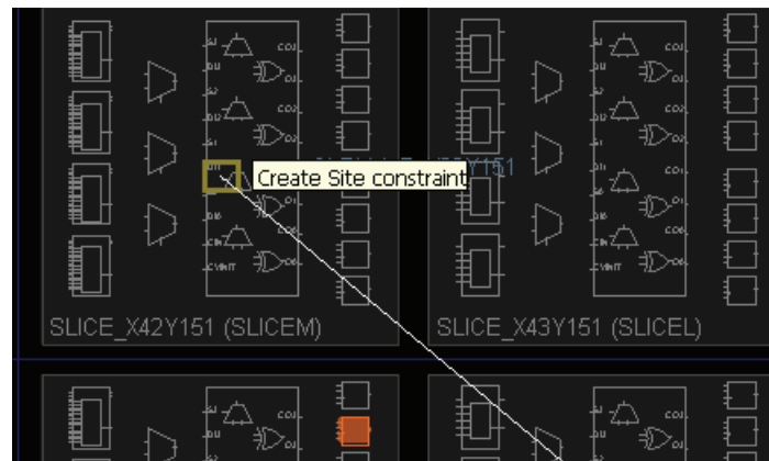
Figure 10-24: Create Site Constraint
