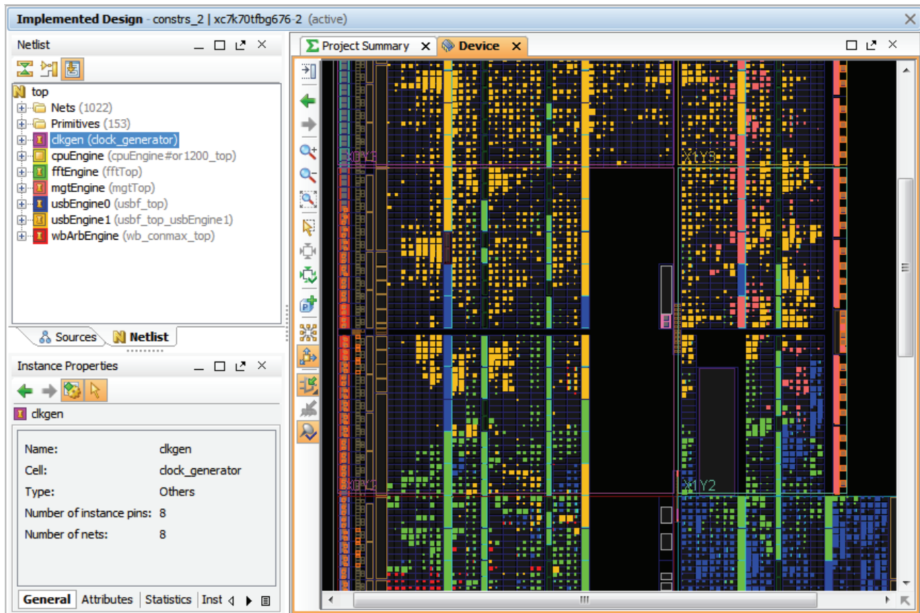
Figure 11-13: Matching Highlighting Color in the Netlist and Device Views
