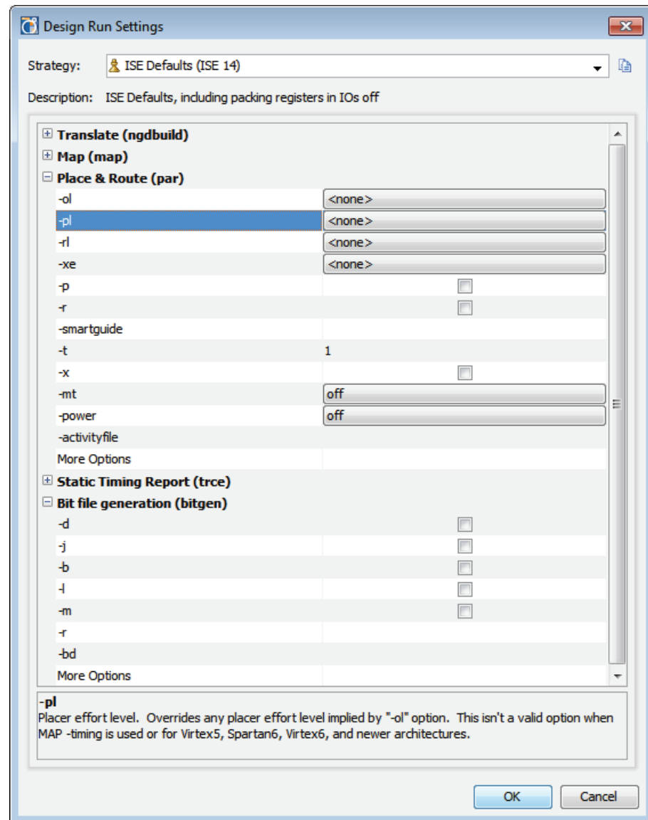
Figure 9-5: Change Implementation Settings
