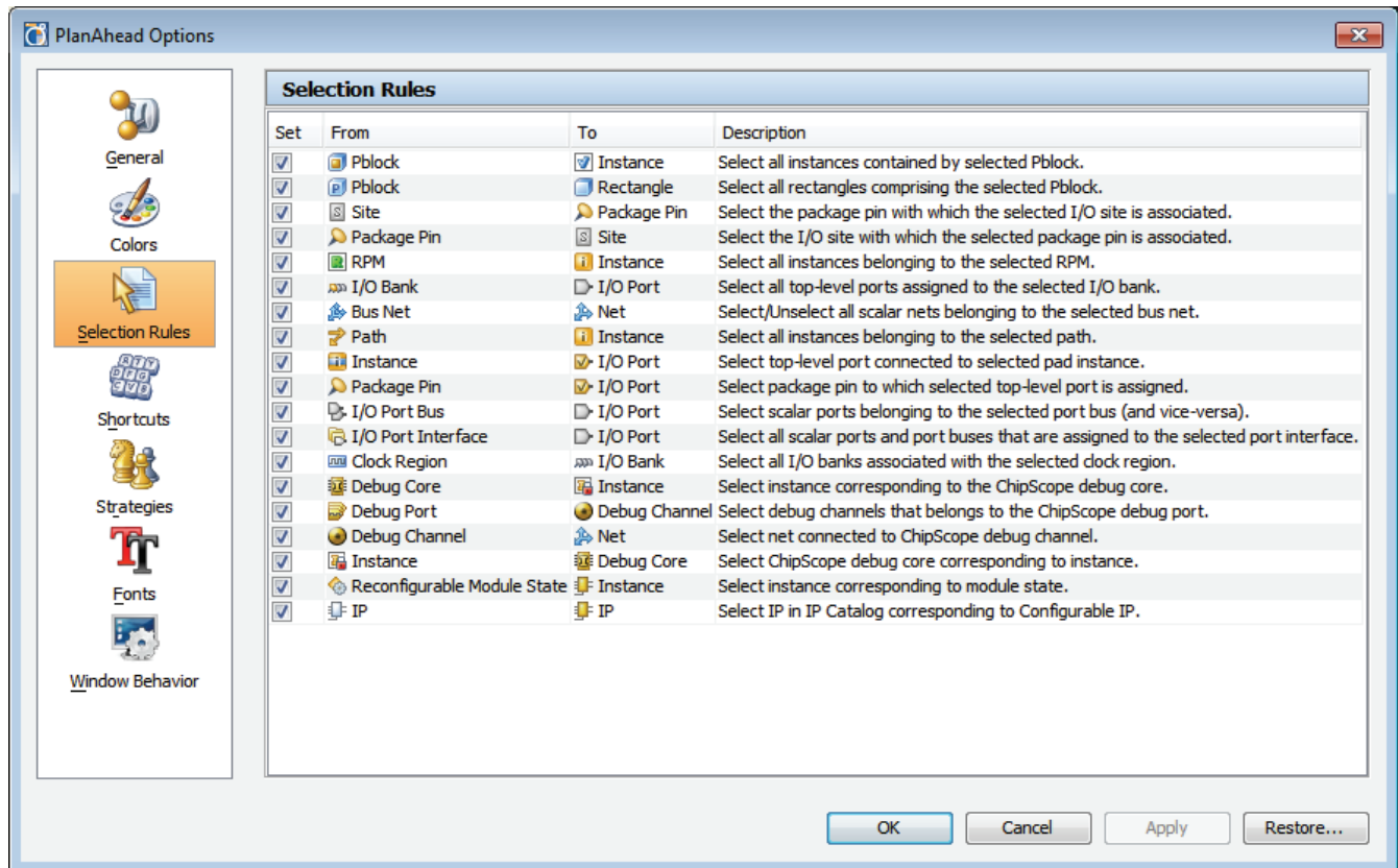
Figure 4-27: PlanAhead Options: Selection Rules
