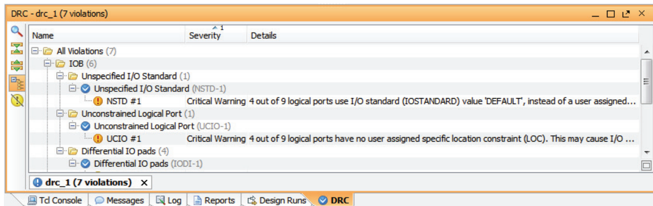
Figure 5-10: Elaborated Design with Objects that Violate DRCs
