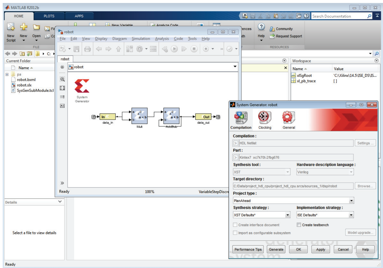
Figure 3-31: Generating DSP Sources in Sysgen
