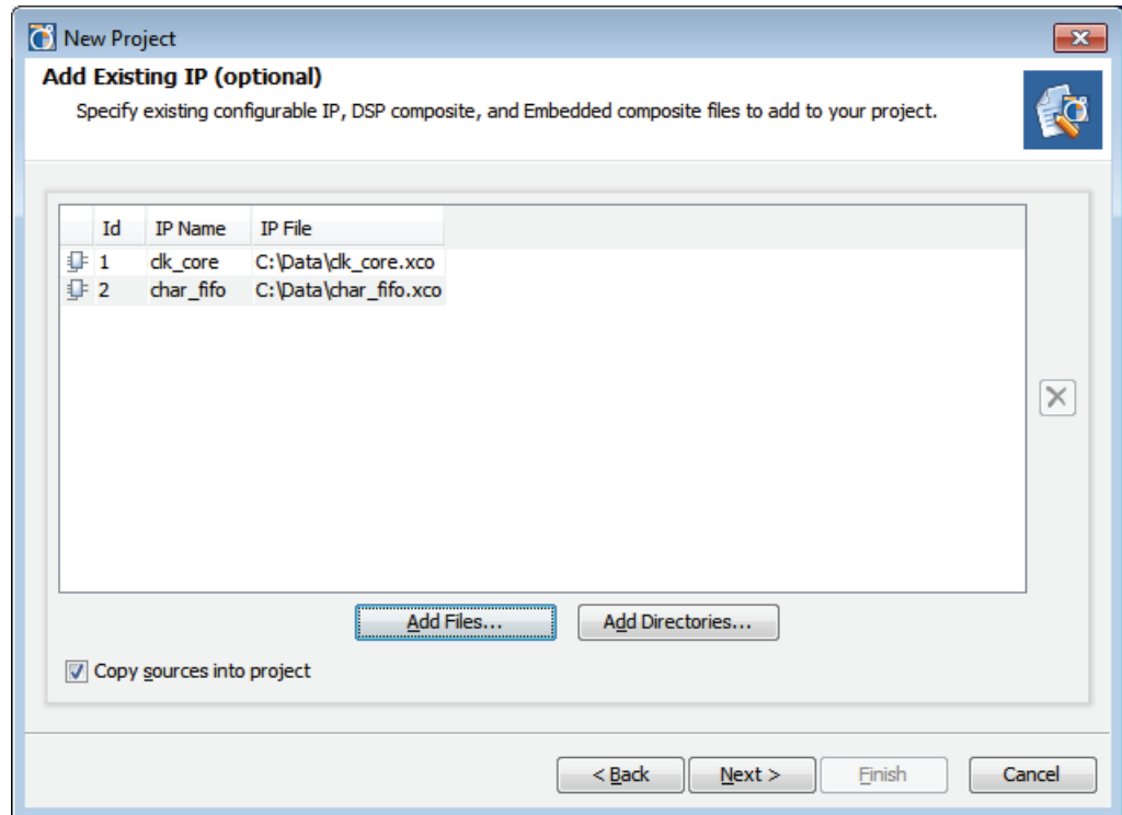
Figure 3-6: Add Existing IP Dialog Box
