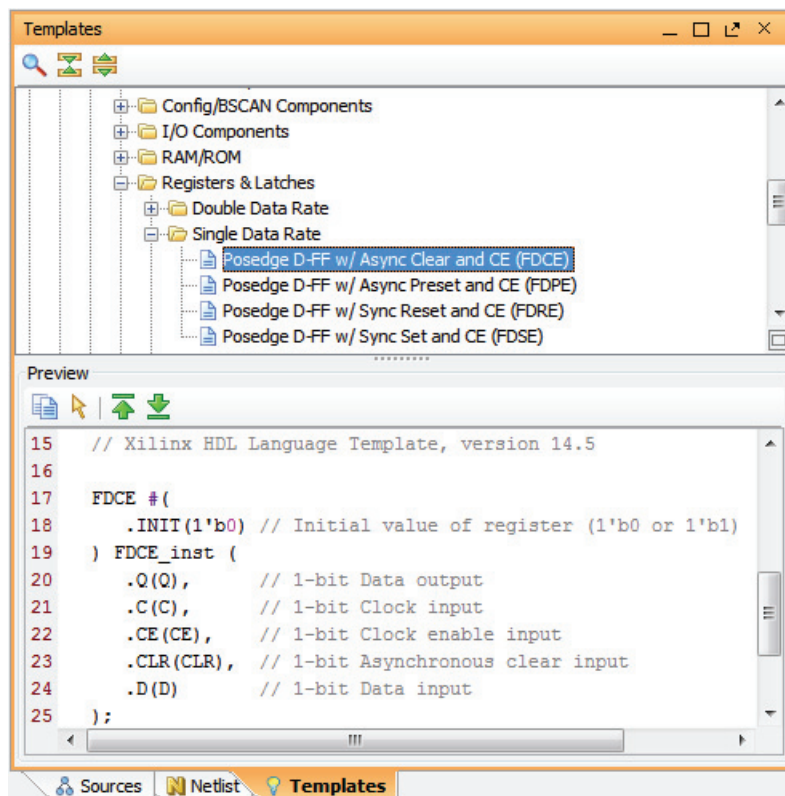
Figure 4-64: Xilinx Language Templates
