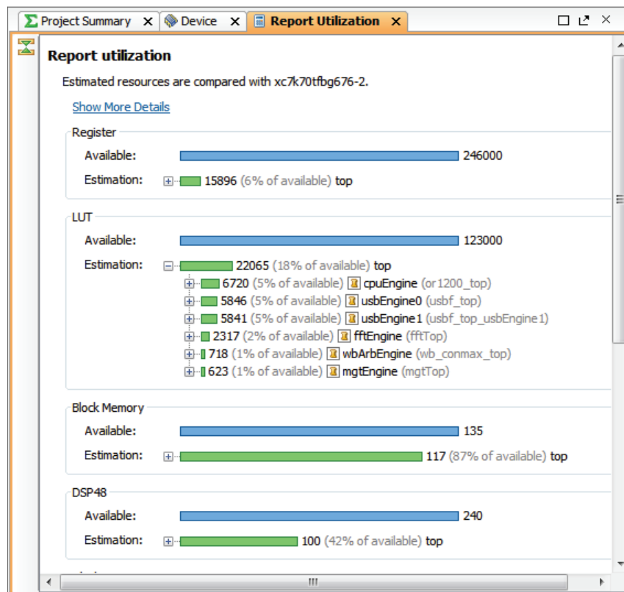
Figure 7-2: Resource Utilization Report
