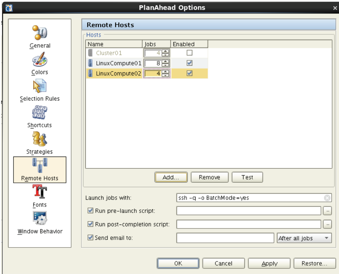
Figure 9-19: Configure Remote Hosts
