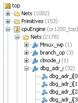
Figure 4-58: Nets Folder in Netlist View
