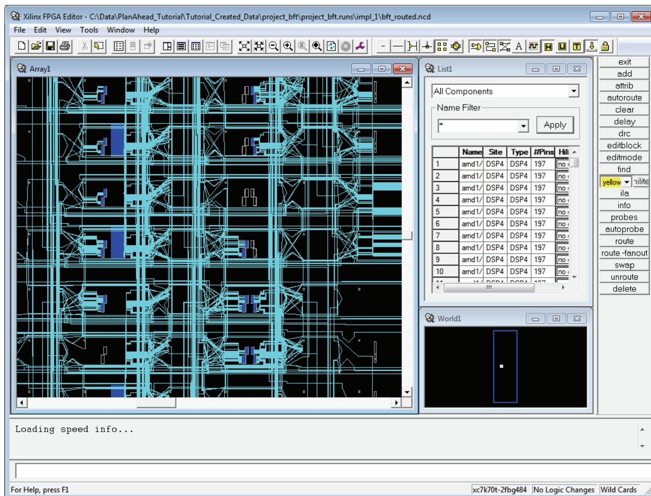
Figure 11-28: FPGA Editor
