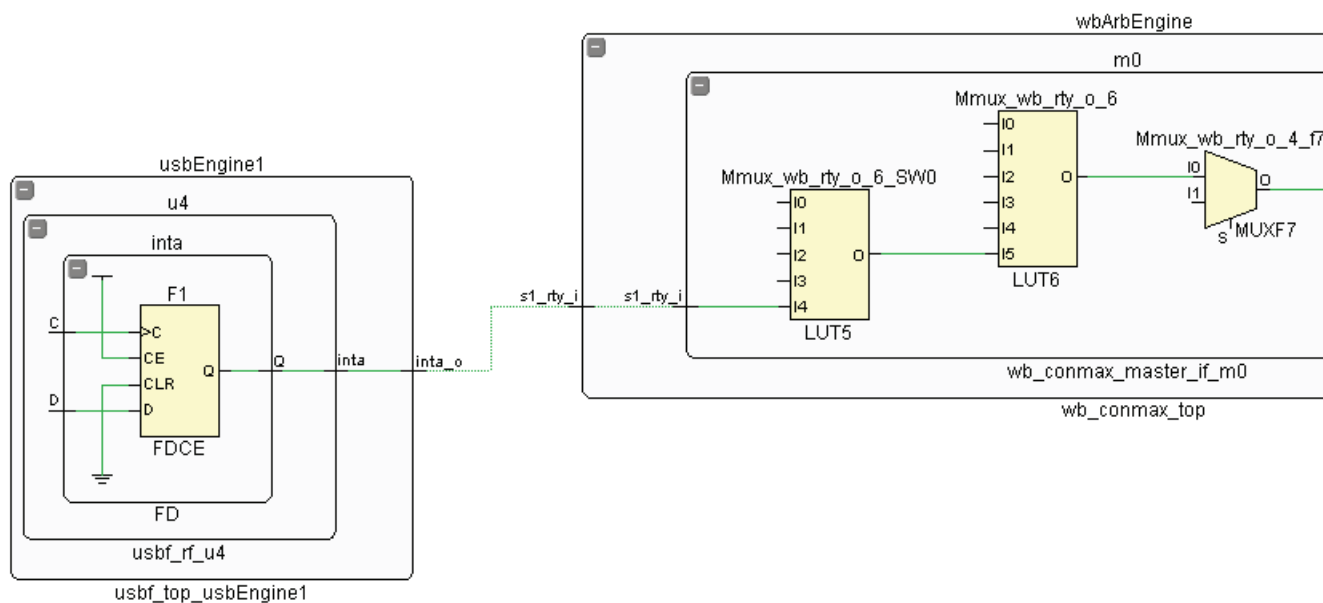
Figure 11-10: Timing Paths Displayed in Schematic View
