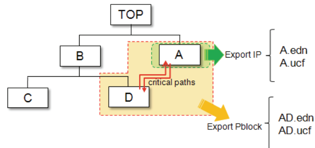
Figure 10-23: Example of Export Pblock and Export IP
