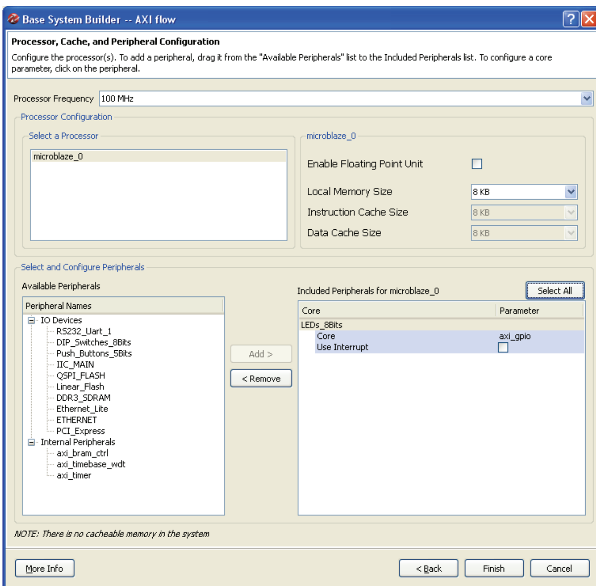
Figure 3-36: Processor, Cache, and Peripheral Configuration
