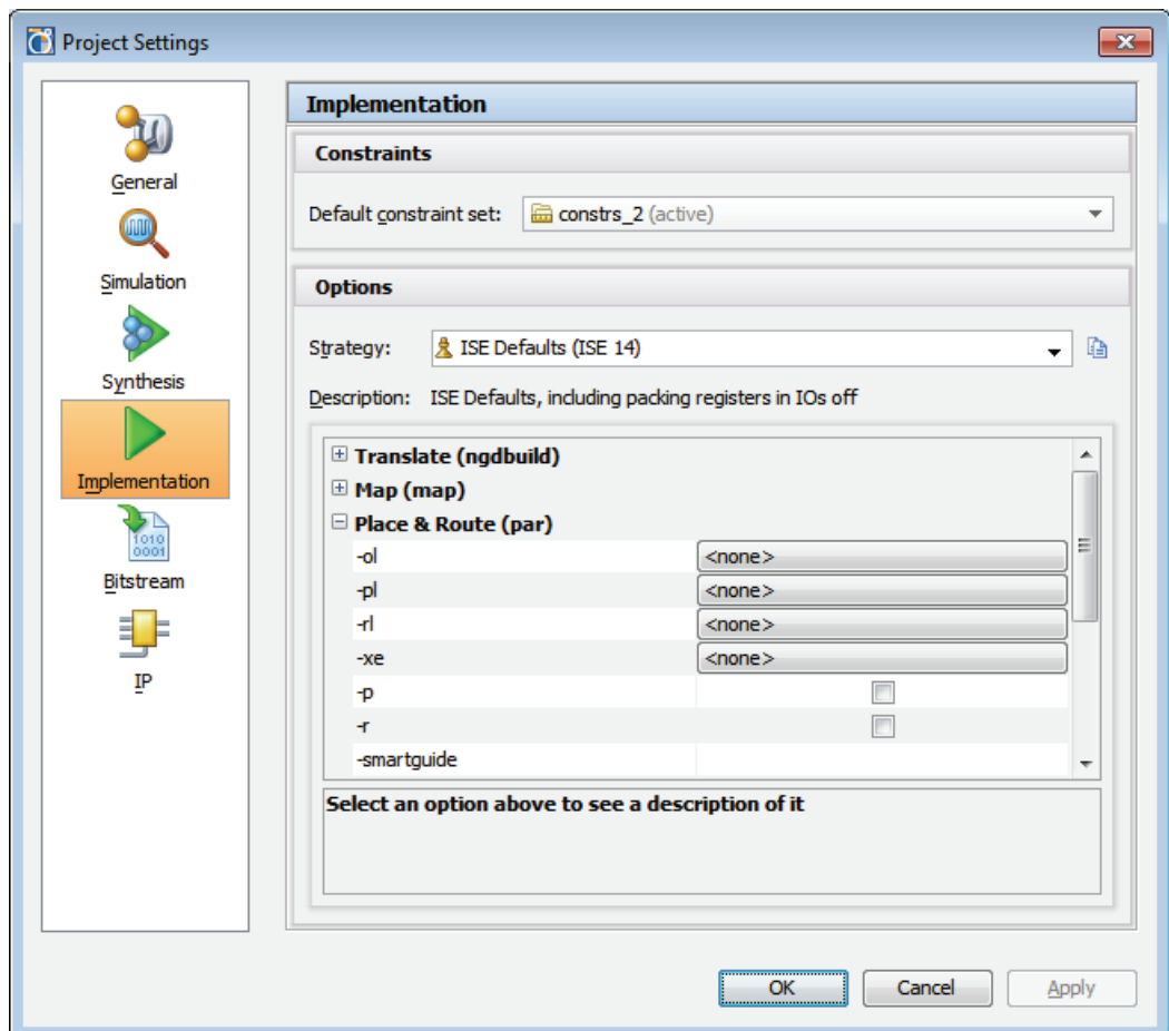
Figure 3-49: Implementation Project Settings
