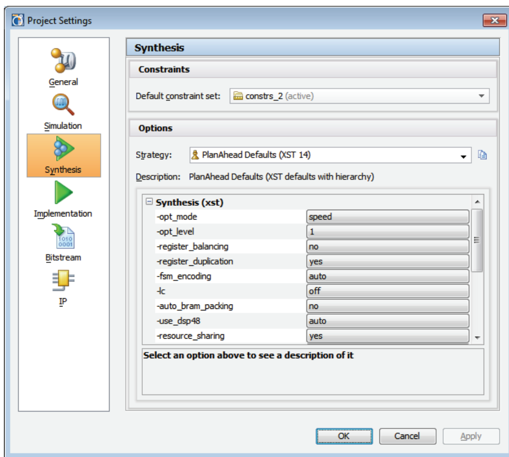
Figure 3-48: Synthesis Project Settings
