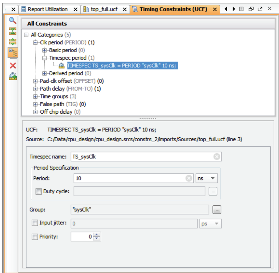
Figure 7-10: Timing Constraints view
