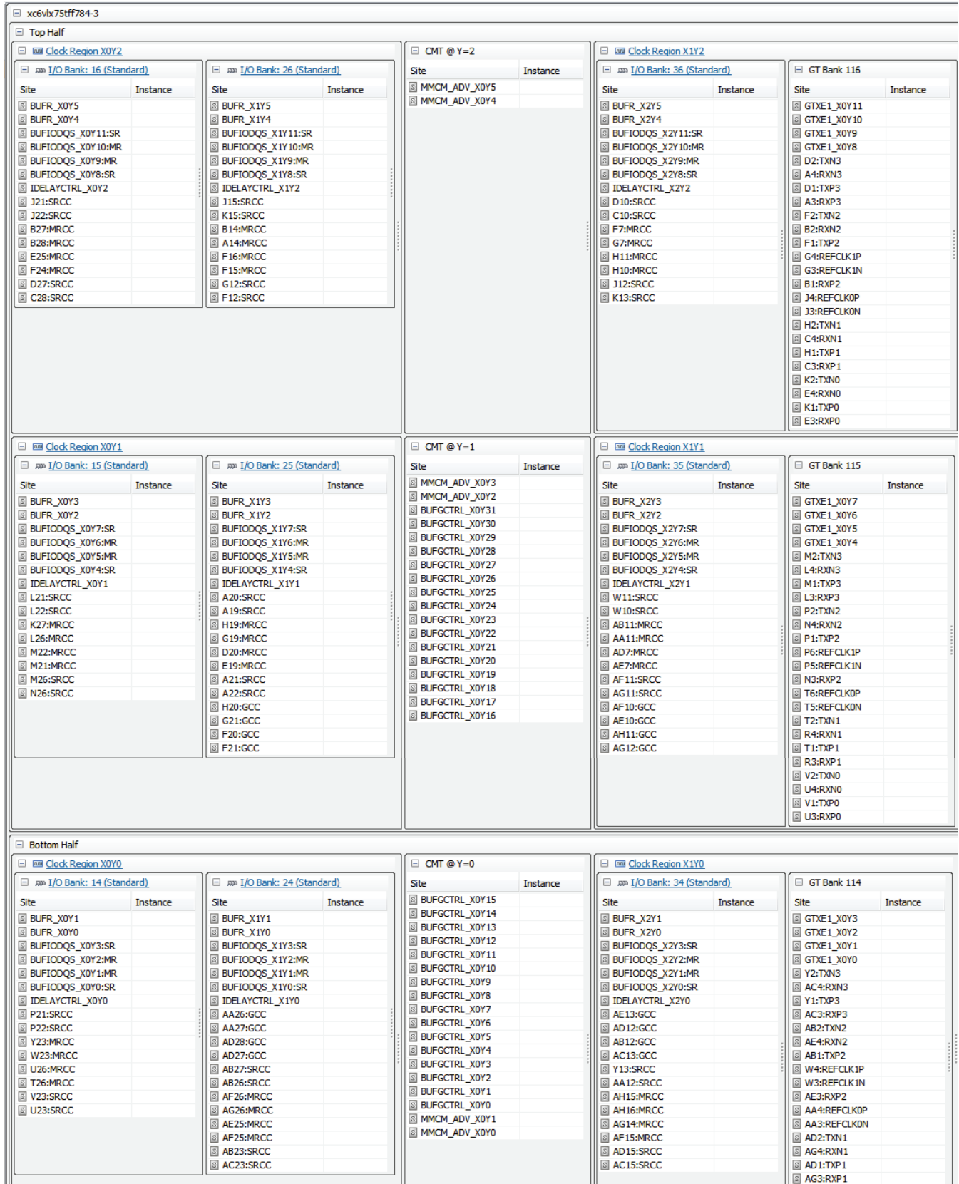
Figure 8-26: Clock Resources View
