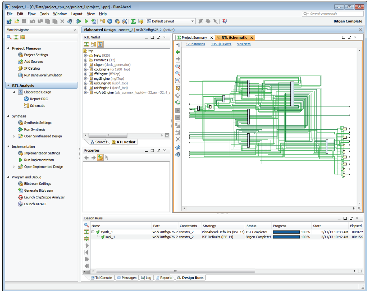
Figure 2-6: RTL Analysis view
