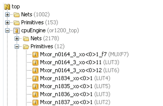
Figure 4-57: Primitives Folder in the Netlist View
