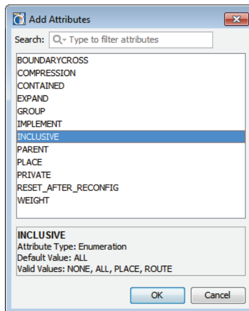
Figure 10-20: Add Predefined Attributes
