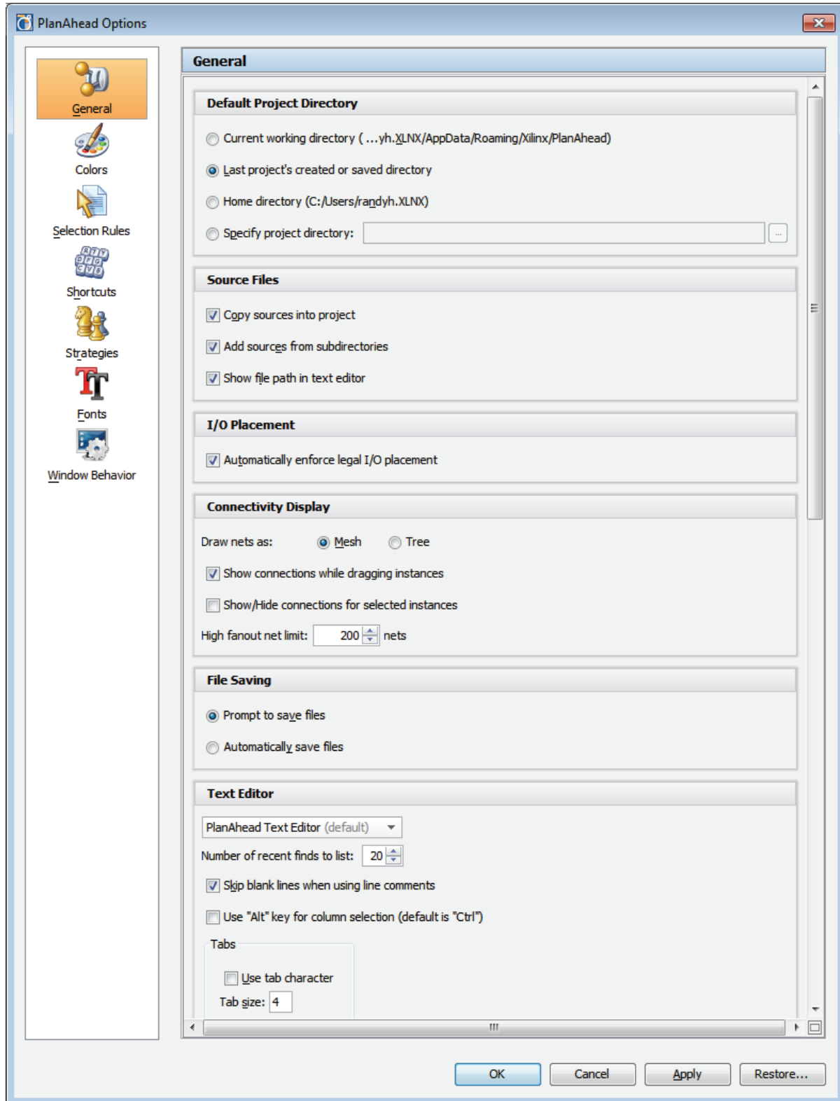
Figure 4-65: General Options Dialog Box
