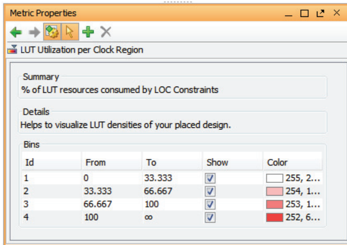
Figure 11-17: Metric Properties View
