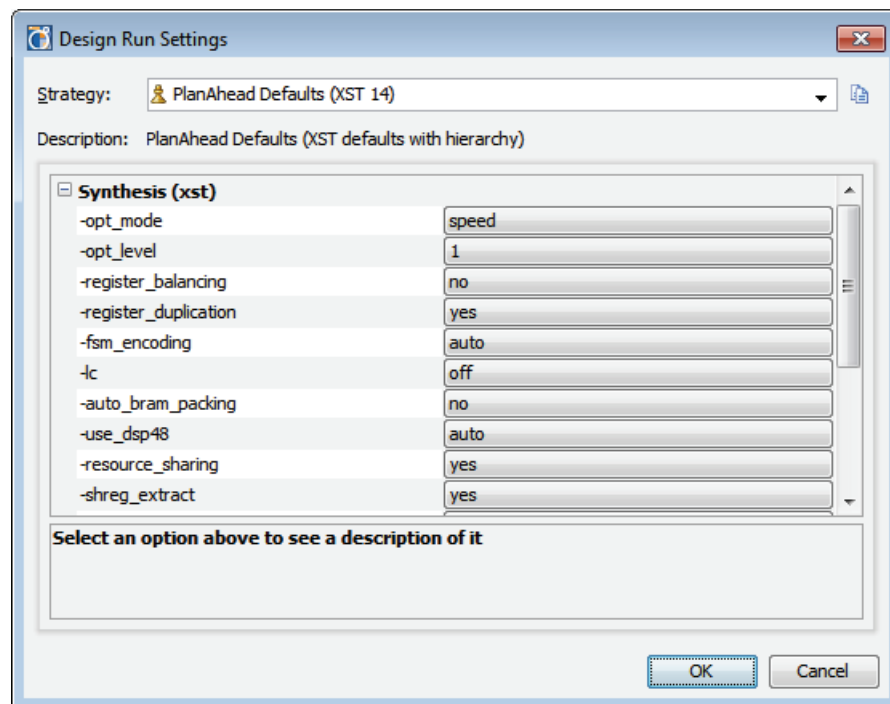
Figure 6-5: Change Synthesis Settings
