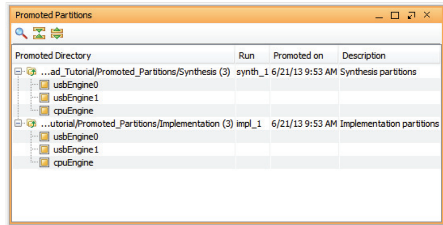
Figure 13-7: Promoted Partitions View
