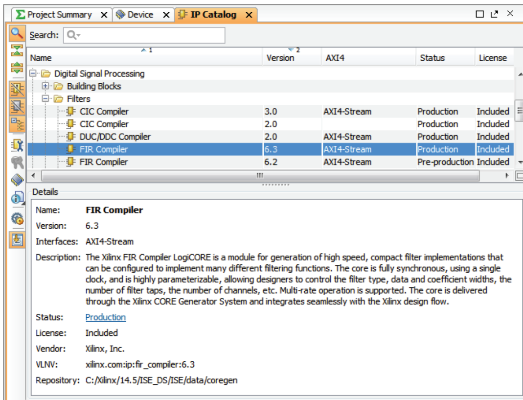
Figure 3-25: Xilinx IP Catalog
