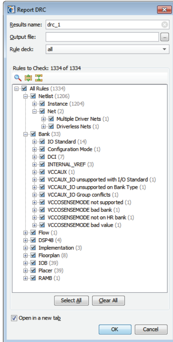
Figure 7-26: Run DRC Dialog Box
