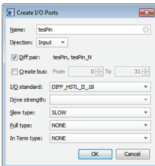
Figure 8-13: Create I/O Ports Dialog Box
