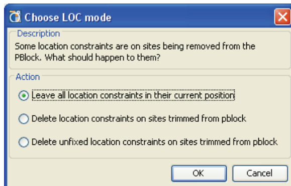
Figure 10-15: Resizing Pblocks with LOCs
