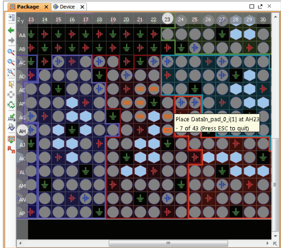
Figure 8-21: Placing I/O Ports Sequentially
